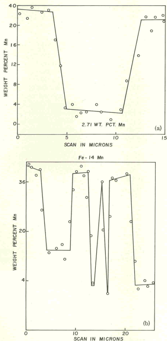
FIG. 6. Electron microprobe data on (a) Fe-7Mn and (b) Fe-14Mn specimens slow cooled and shock loaded at 300 kbar.
