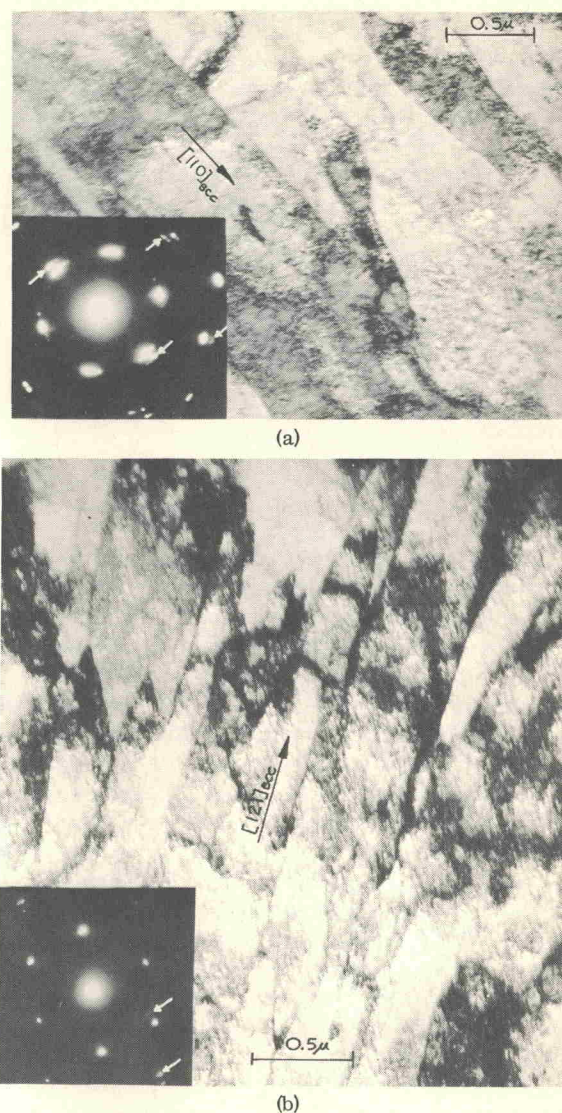
FIG. 7. (a) Electron micrograph of quenched shock-loaded Fe-7Mn at 90 kbar. The fcc plates have transformed from the initial bcc structure. The fcc plates have been identified by electron diffraction. (b) Electron micrograph of slow-cooled shock-loaded Fe-7Mn at 90 kbar.
